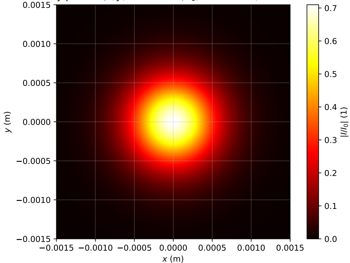
Intensity profile I(x, y, z = 2.866m)/I_0 , Pin=0.6Pcr, artificial time
